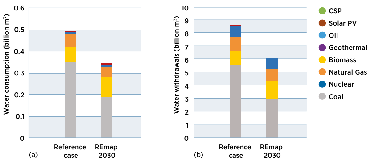
Figure A.3 Projected water (a) consumption and (b) withdrawals under Reference Case and REmap 2030 for Germany
