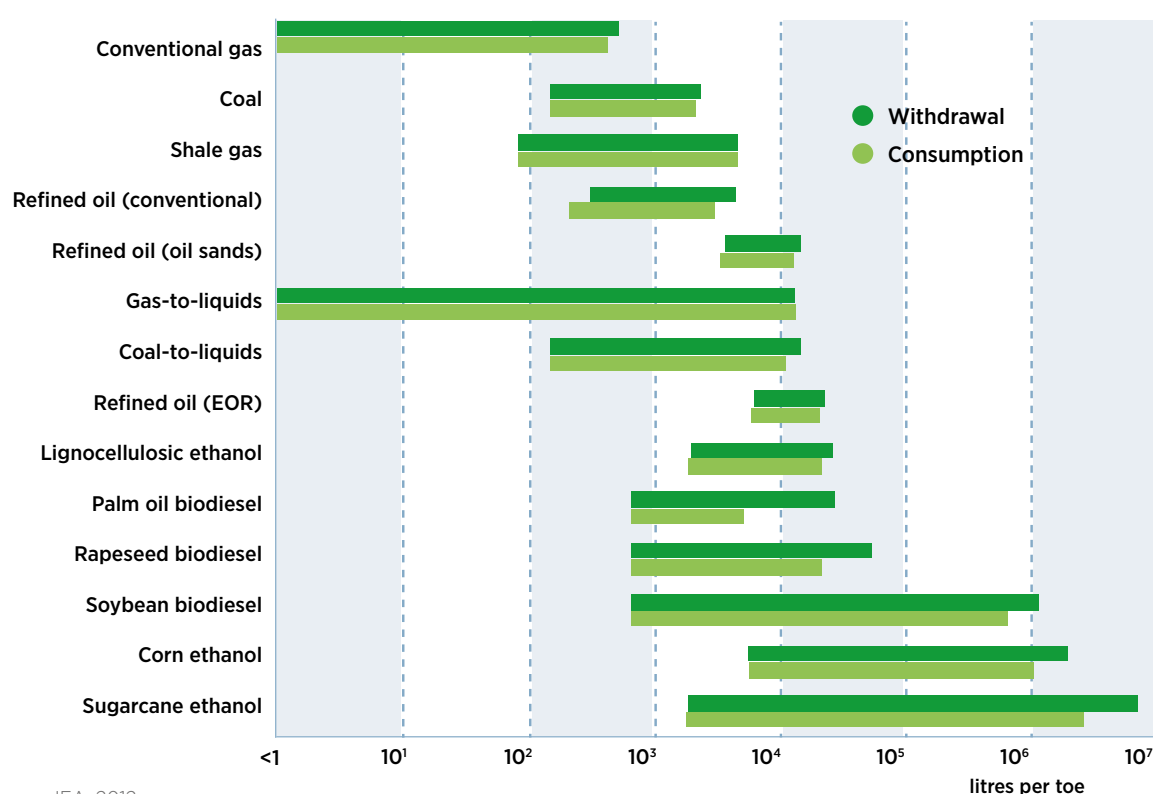
Figure 2.11 Water withdrawal and consumption for primary fuel extraction, processing and transportation
