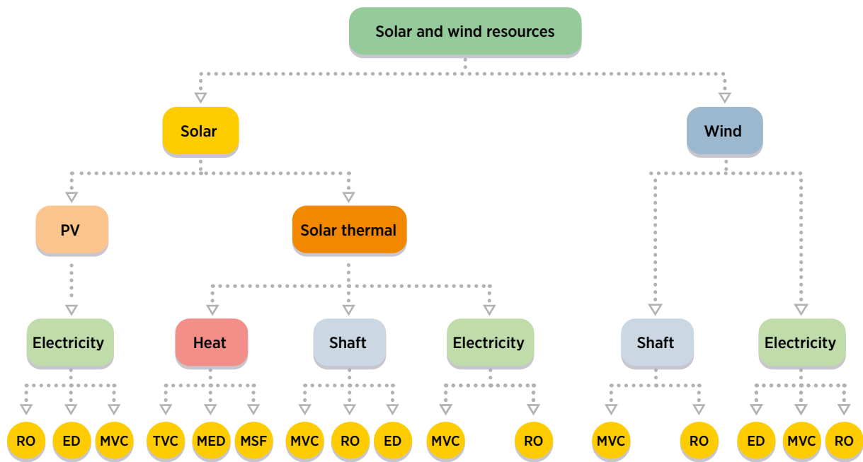
Figure 2.4 Pathways for integrating solar and wind resources with different desalination technologies
