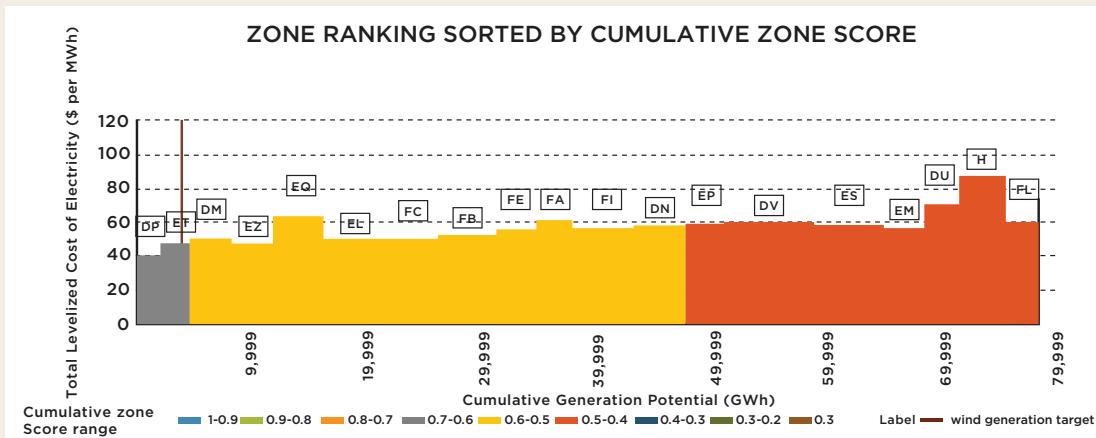
Figure 21: Zone ranking sorted by levelised cost of electricity (above) and by cumulative zone score
